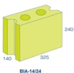
BIA-14/24
