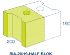
BIA-20/19-HALF BLOK
