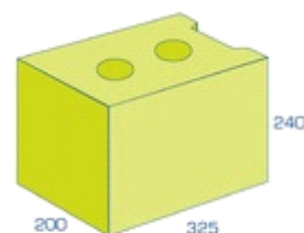
BIA-20/24-HOEKBLOK
