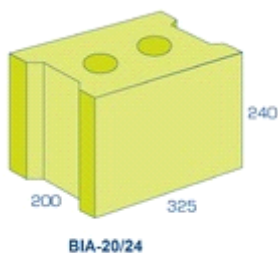
BIA-20/24
